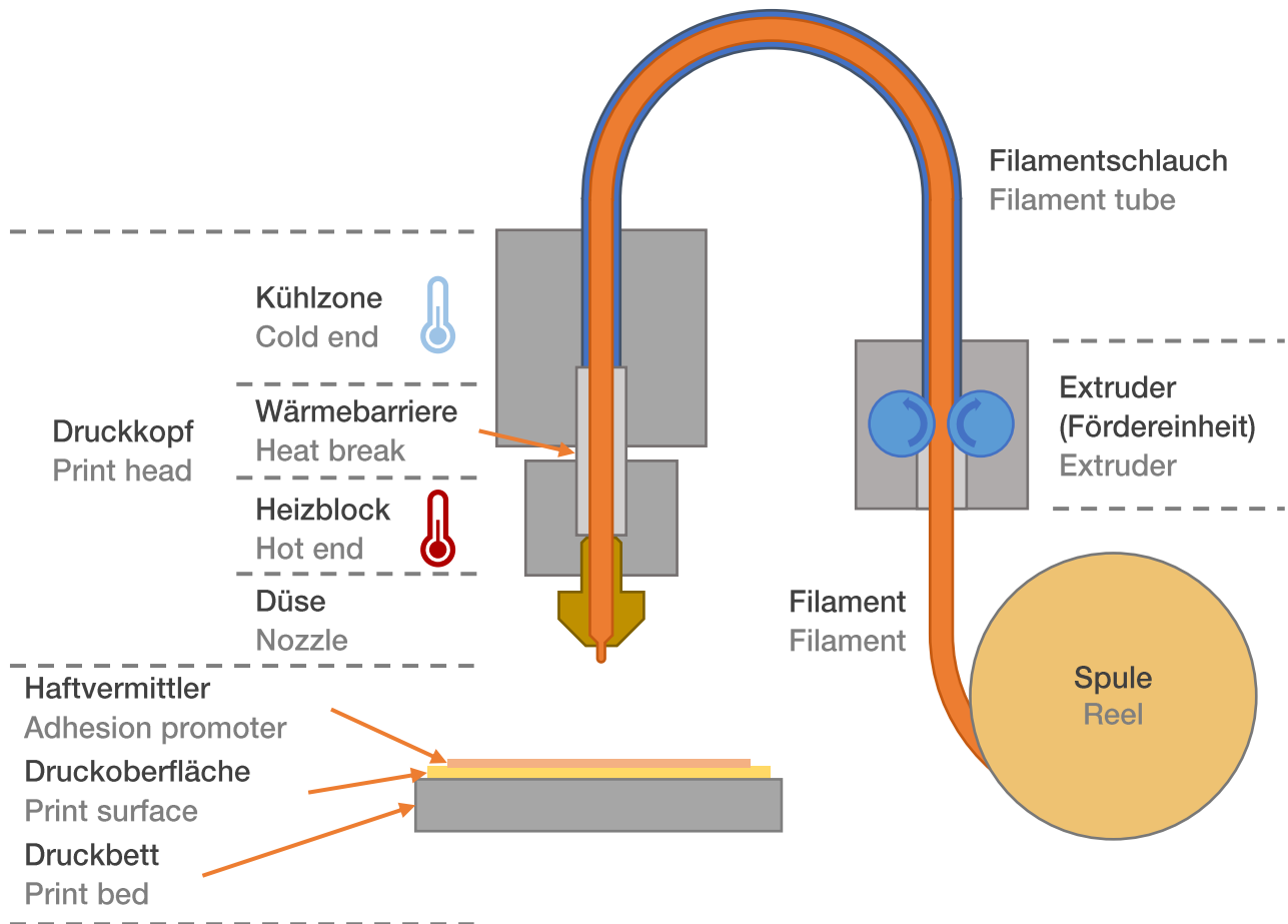
1: Schema Filament-3D-Drucker – Filament 3D printer schematic
