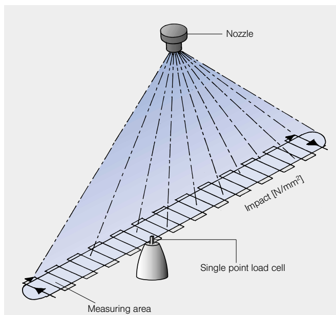
Measuring principle
