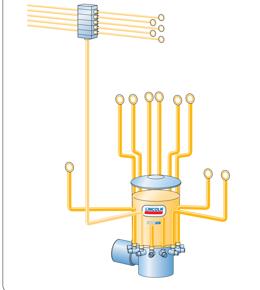
Schematic multi-line system
