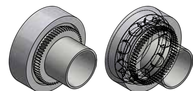
Gear-driven shaft: one-part solution for full integration
