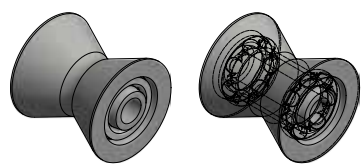
Guide roller for rubber seals in car production: which replaced a special unavailable roller
