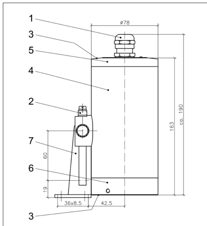
Dimensions for Lumistar luminaires ASL 55-LED and ESL 55-LED
