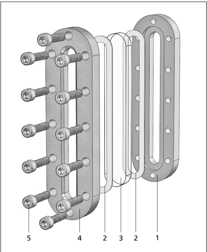
Exploded view of a Lumiglas oblong oval sight glass fitting
