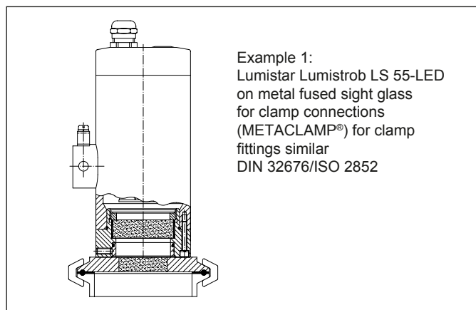
Lumistar Lumistrob LS 55-LED
