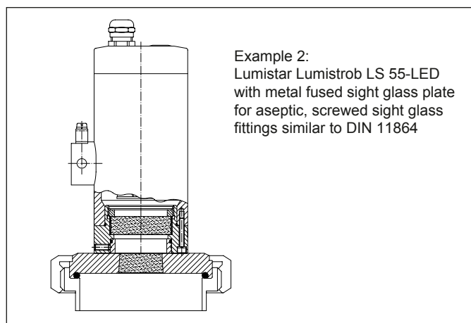
Mounting options
