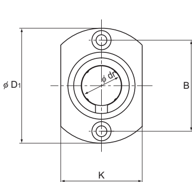
Models LMCH 6L to 13L
