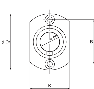
Models LMIH 6L to 13L
