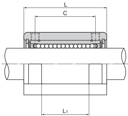
A arrow view Model SC35
