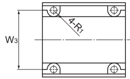
A arrow view Model SC40 and SC60
