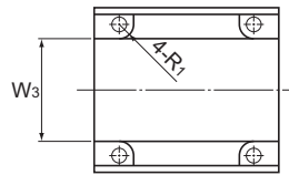
A arrow view Model SC35
