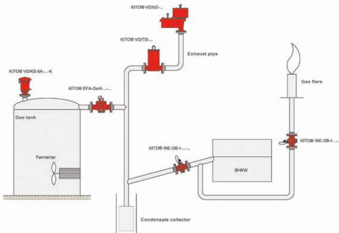
Fig. 2: Exemplary protection concept of an agricultural biogas plant
