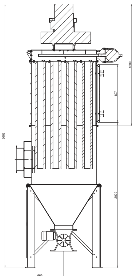
View B-B
