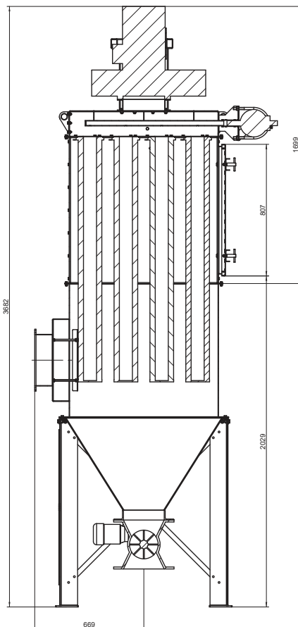
View B-B
