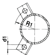
DN 125 – 150
