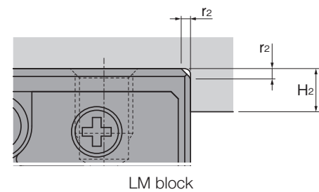
LM block
