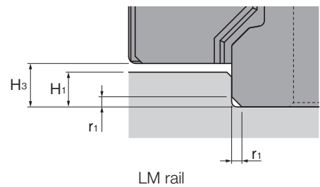
LM rail
