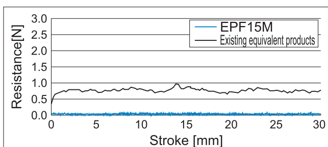
Fig.2 Comparison of rolling resistance test data
