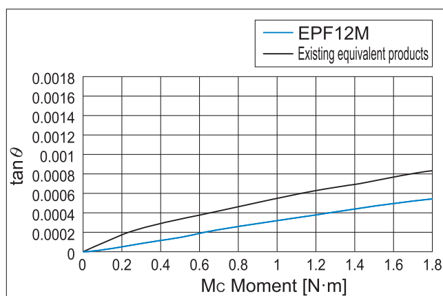
Fig.1 Comparison of M_c moment test data
