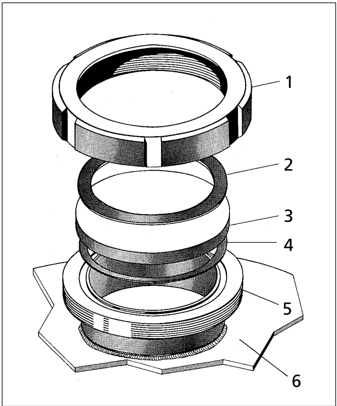
Exploded view of a Lumiglas screwed sight glass fitting MV
