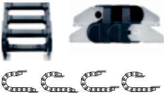
Possible installation conditions - Further installation angles ► installation sketch
