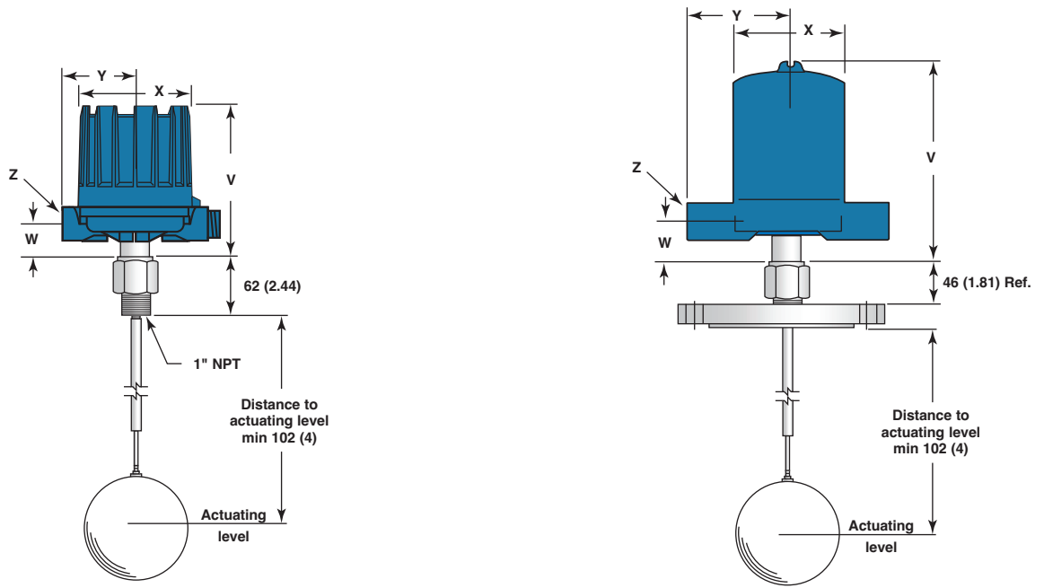
Model T20 with 1" NPT
