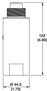
705/706 Adapter
