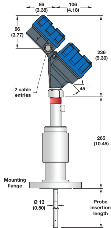
Model 7yN with flanged connection
