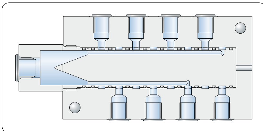
EFM-metering device – inlets
