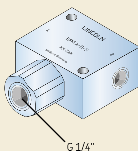
EFM-metering device – inlets
