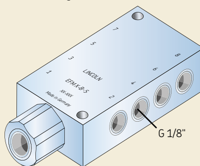
EFM-metering device – outlets
