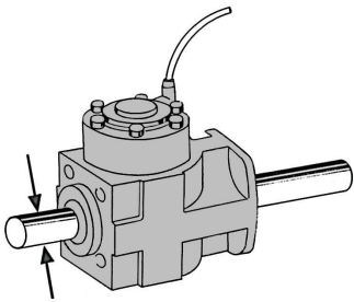
For chrome-plated rods Shafts with F8-F7 tolerance are to be used
