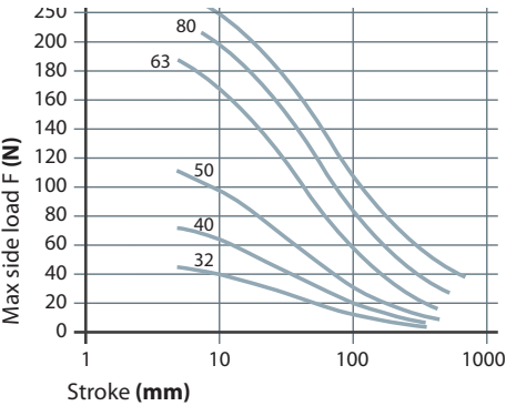
Standard piston Ø32 ÷ 63 mm
