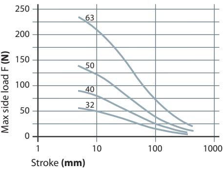
Long piston Ø32 ÷ 63 mm
