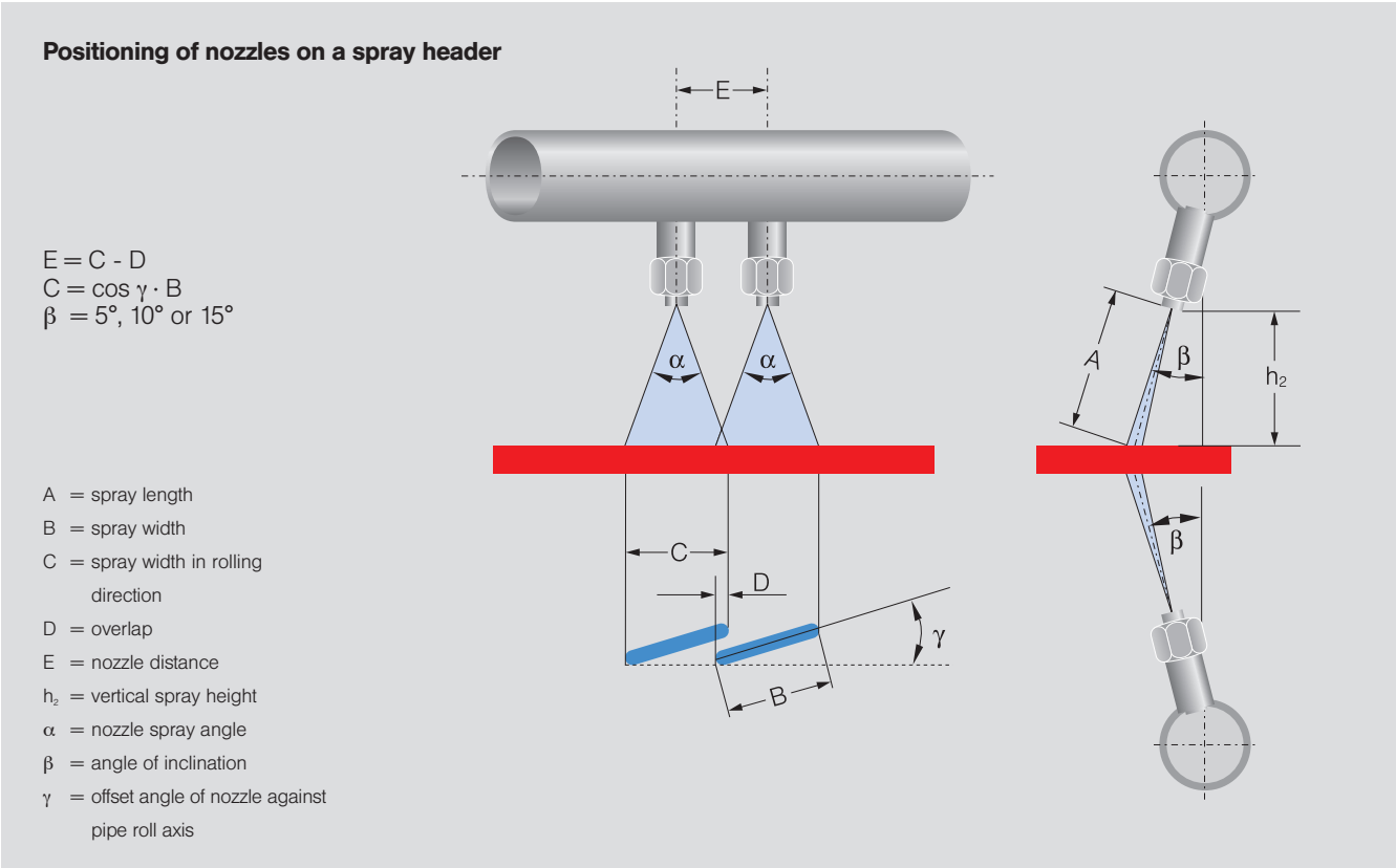
Spray length (A), spray width (B, C), overlapping (D), nozzle distance (E) with vertical spray height ( h_2 ), nozzle spray angle ( \alpha ) and angle of inclination ( \beta )
