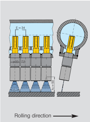
Possible arrangement of welding nipples for MiniSCALEMASTER® HP (with hexagonal socket)
