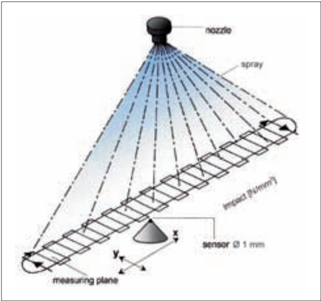
Measuring principle
