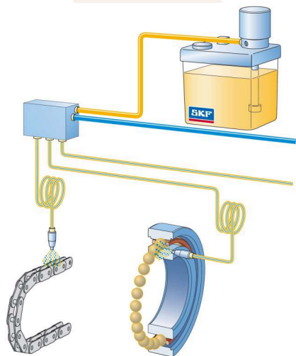
obr: systém SKF Air+Oil
